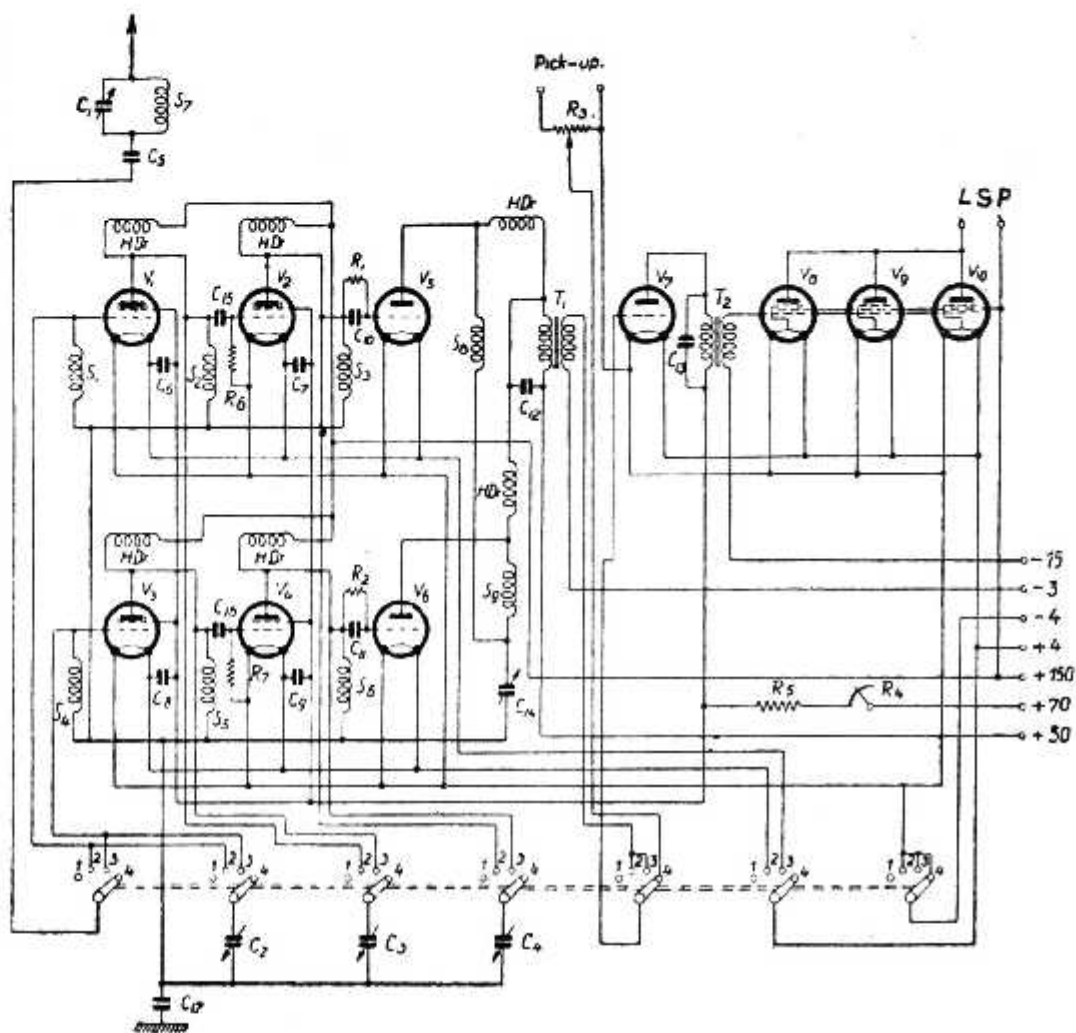
Principle-schematic.
